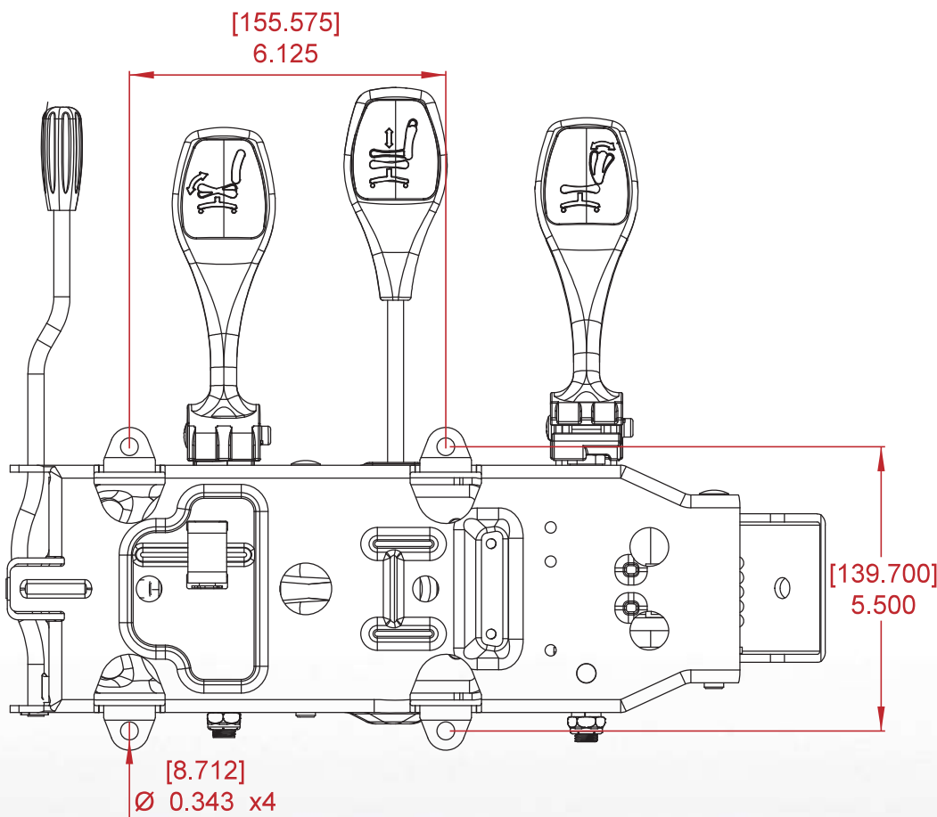
Seat Plate Mounting View
